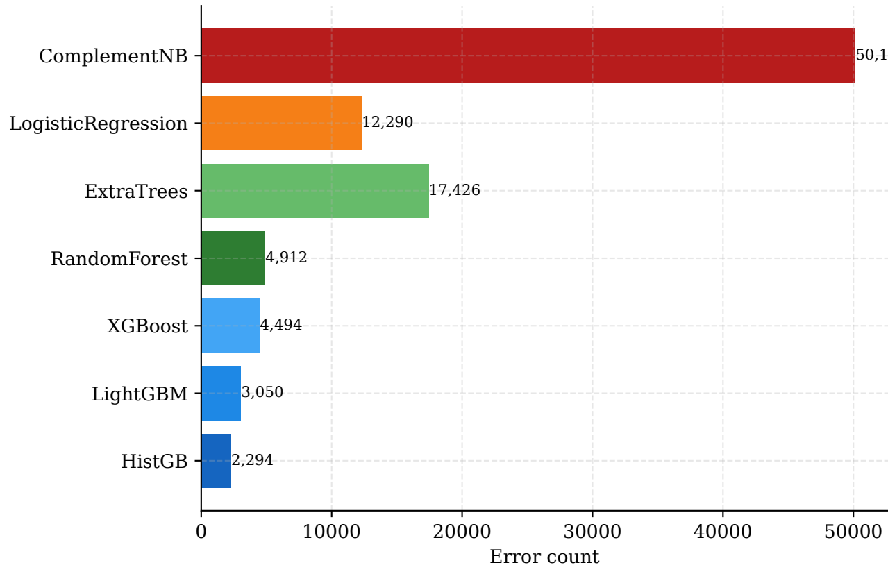
Misclassification Count — fold 2
