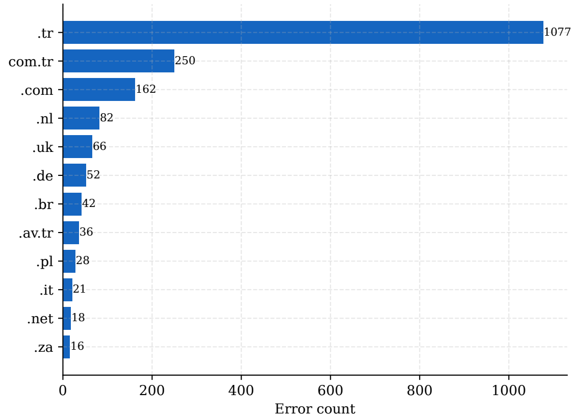
HistGB Errors by TLD — fold 2
