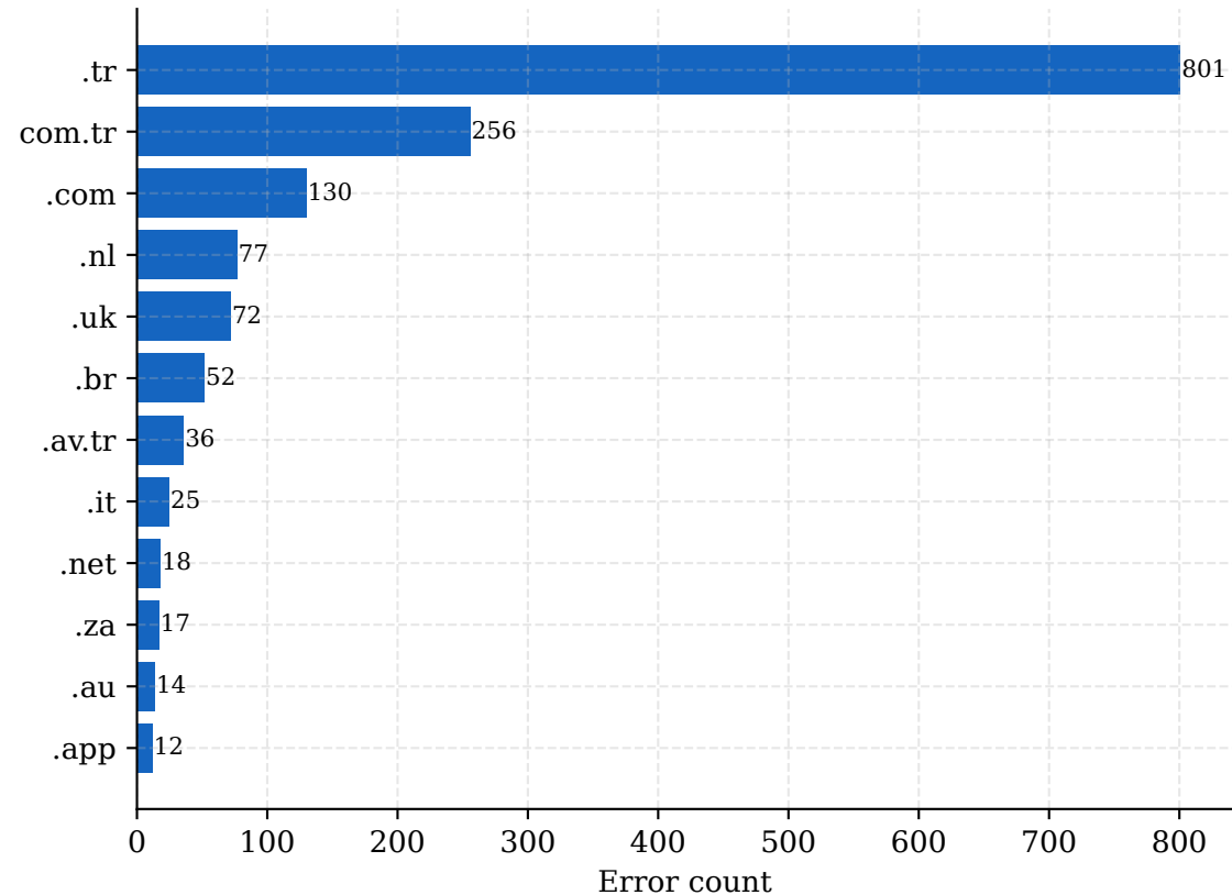
HistGB Errors by TLD — fold 3
