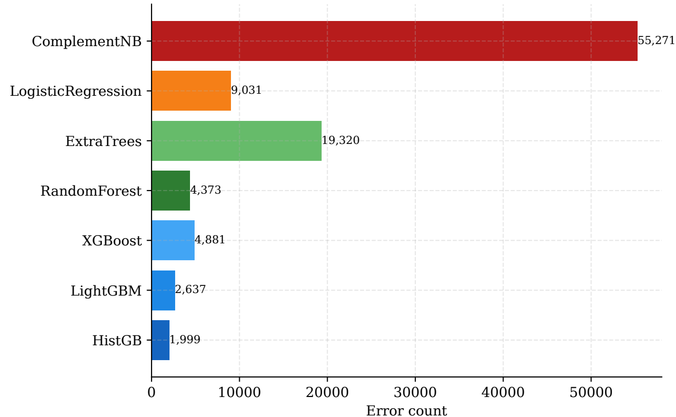
Misclassification Count — fold 3
