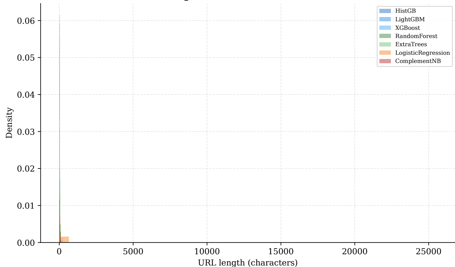
URL Length of Misclassified URLs — fold 3
