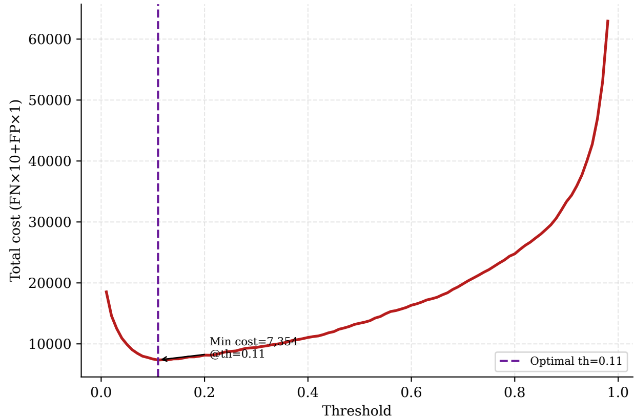
Cost-Sensitive Analysis
