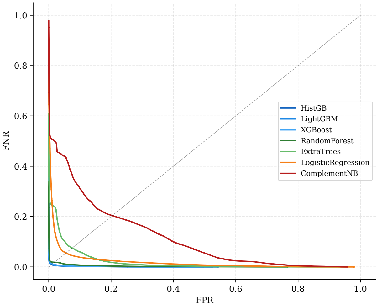
DET – fold 0
