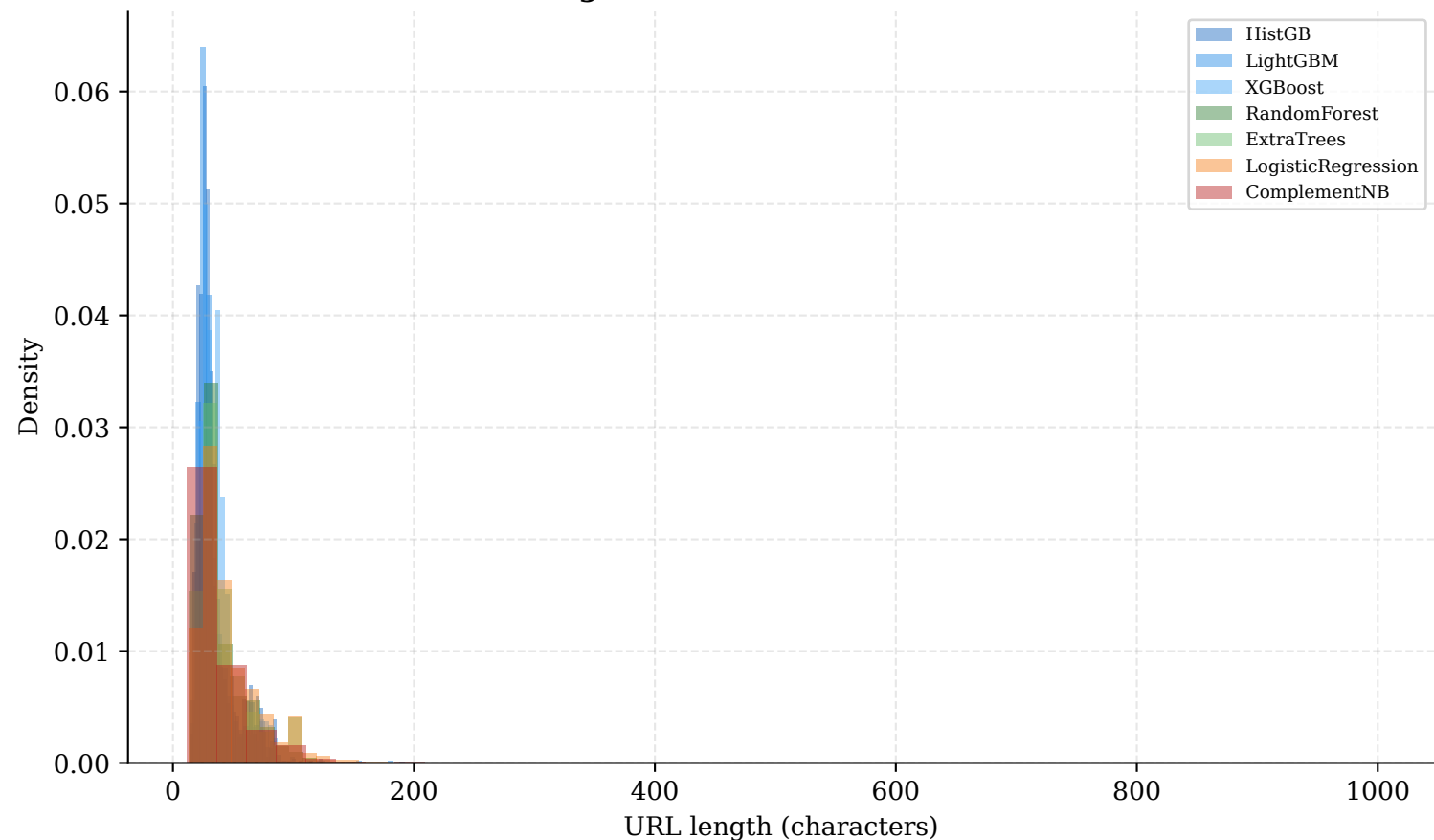
URL Length of Misclassified URLs — fold 0
