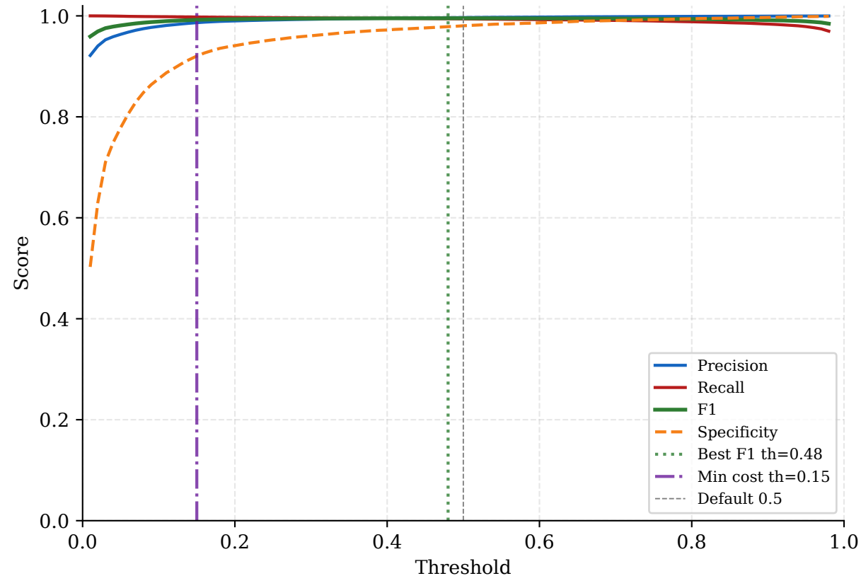
Threshold Sensitivity — HistGB fold 0
