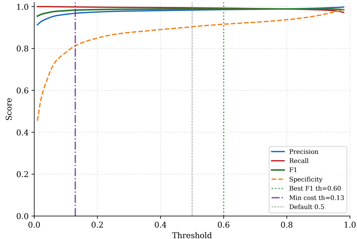
Threshold Sensitivity — HistGB fold 1
