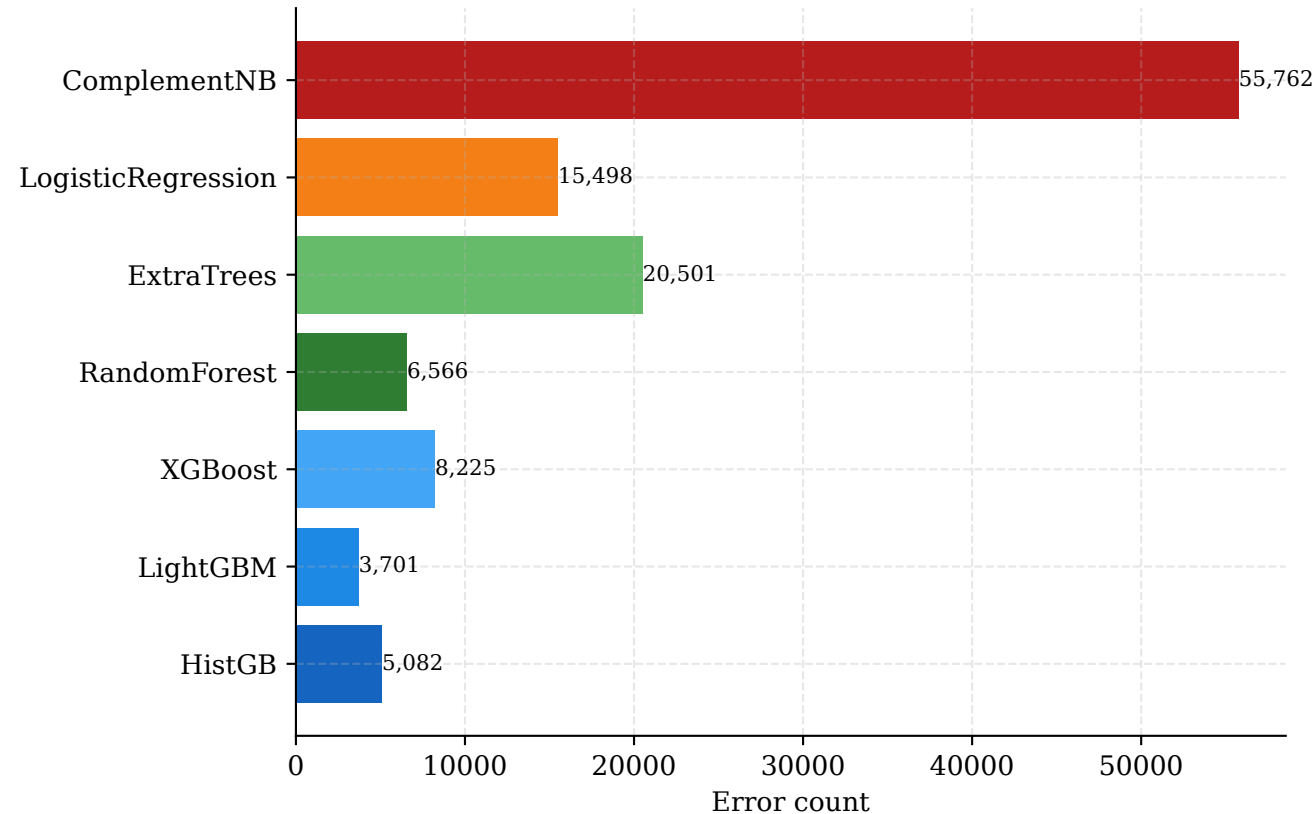
Misclassification Count — fold 4
