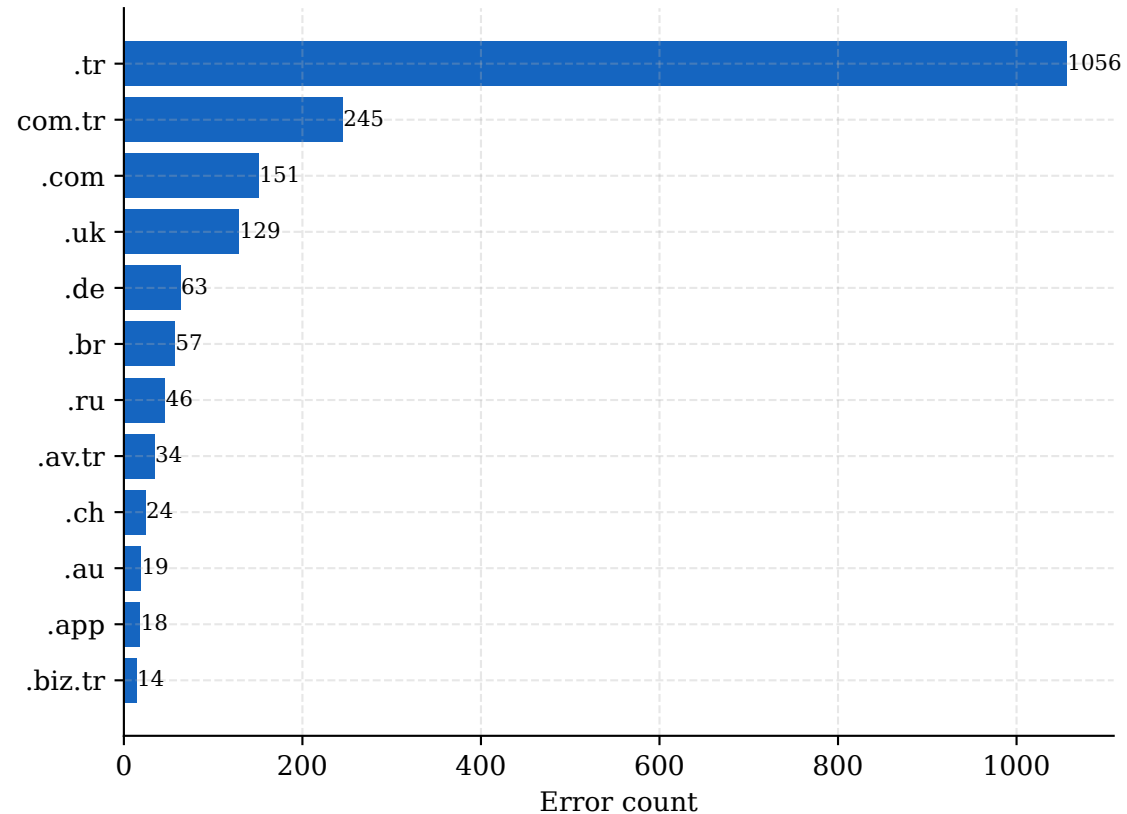
HistGB Errors by TLD — fold 4
