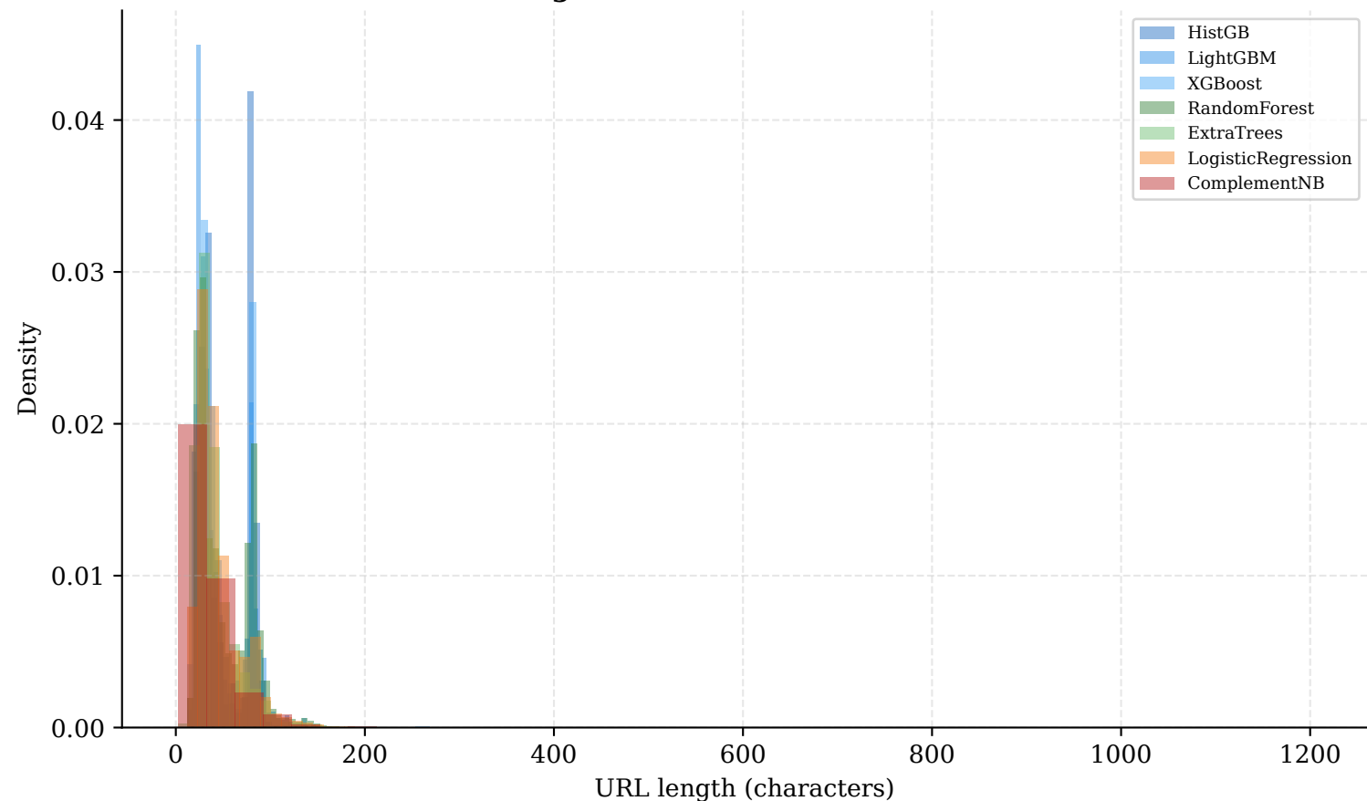
URL Length of Misclassified URLs — fold 4
