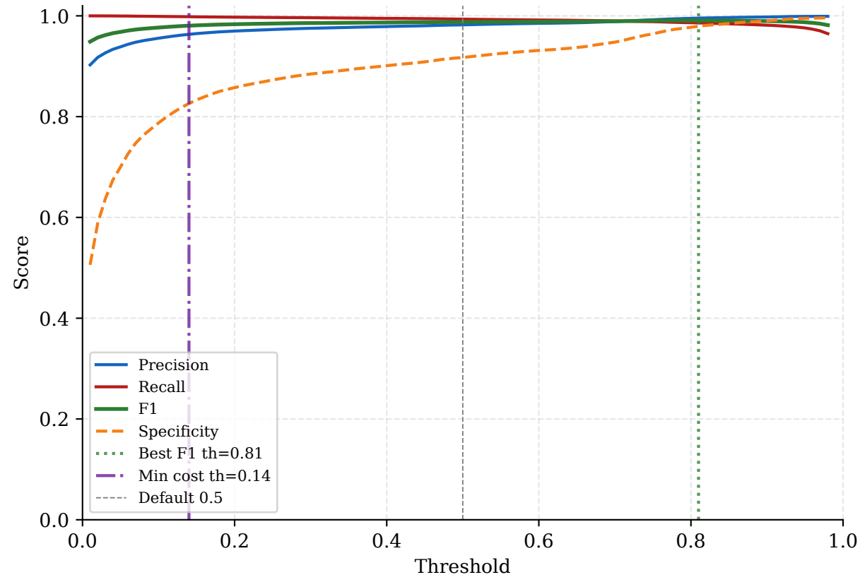
Threshold Sensitivity — HistGB fold 4
