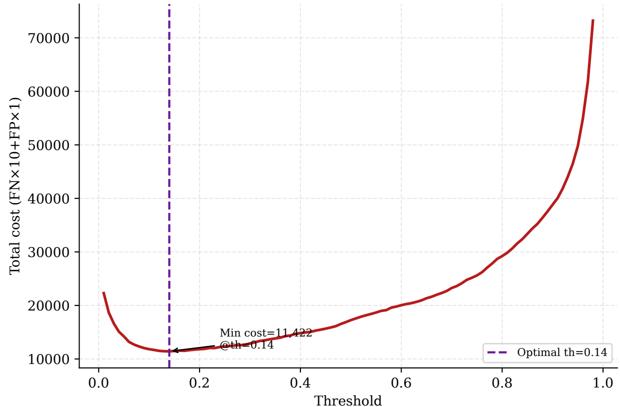
Cost-Sensitive Analysis
