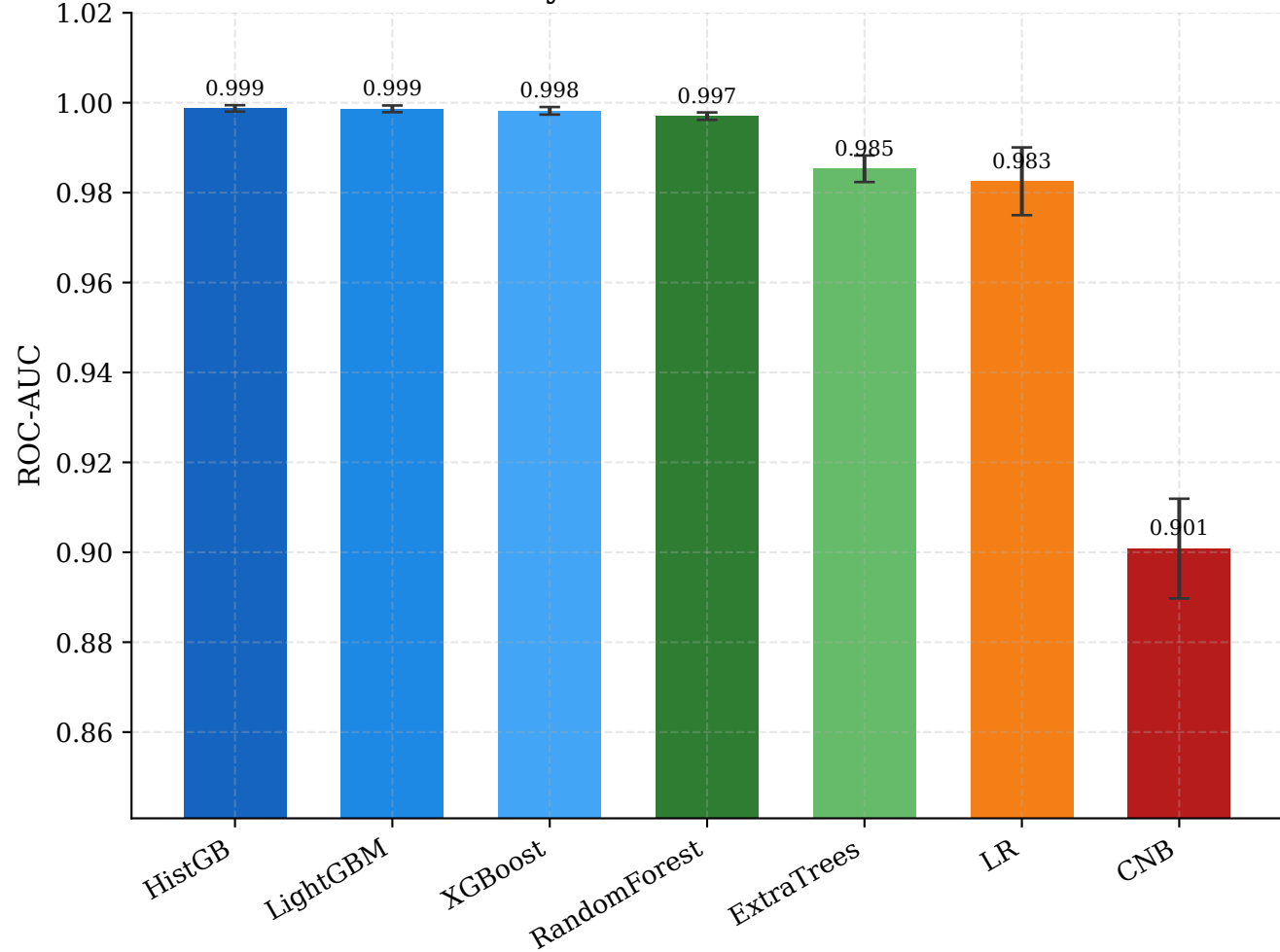
Binary Detection — 5-Fold CV
