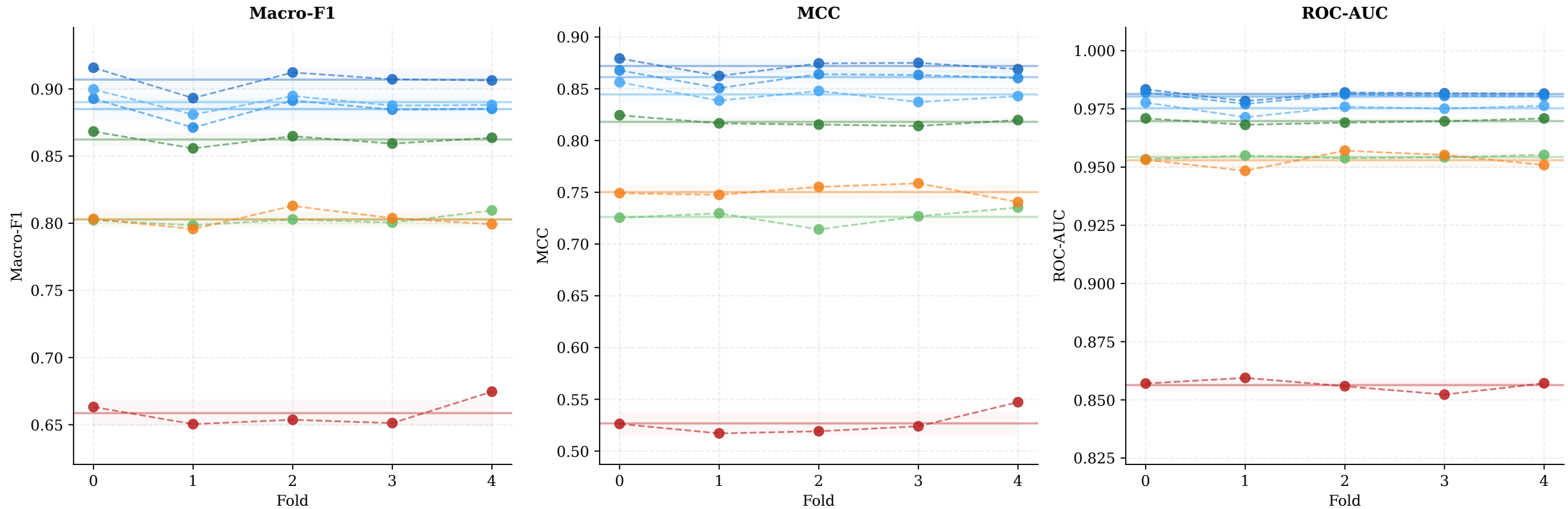
Performance per Fold — 5class task (scatter=individual fold; dashed line=trajectory; shaded= \pm 1 std band)
