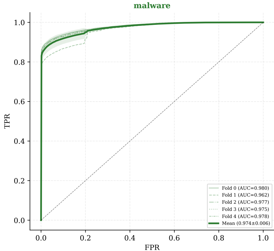
HistGB — Per-Class ROC Curves (5class, all 5 domain-insulated folds)
