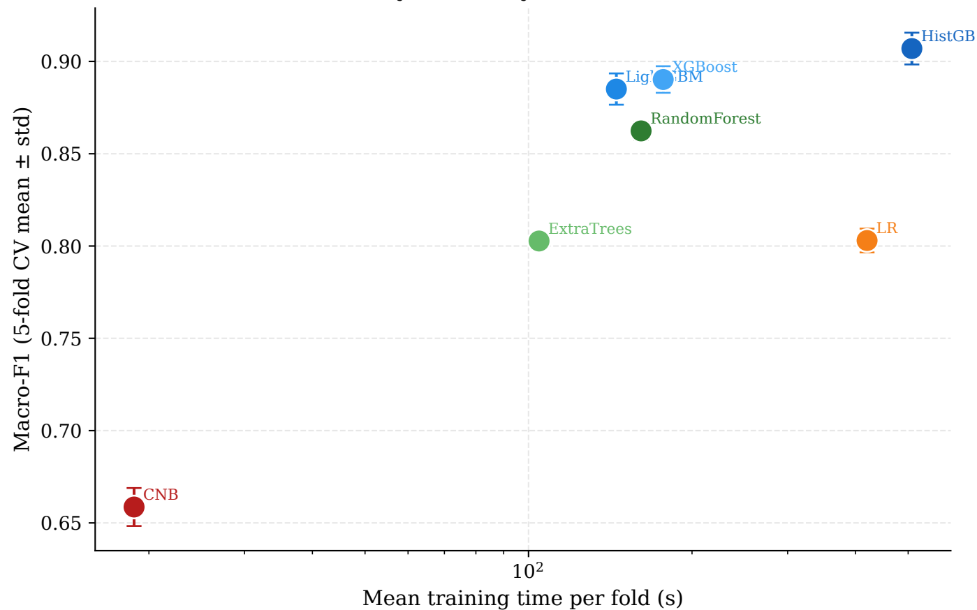
Accuracy-Efficiency Tradeoff — 5class
