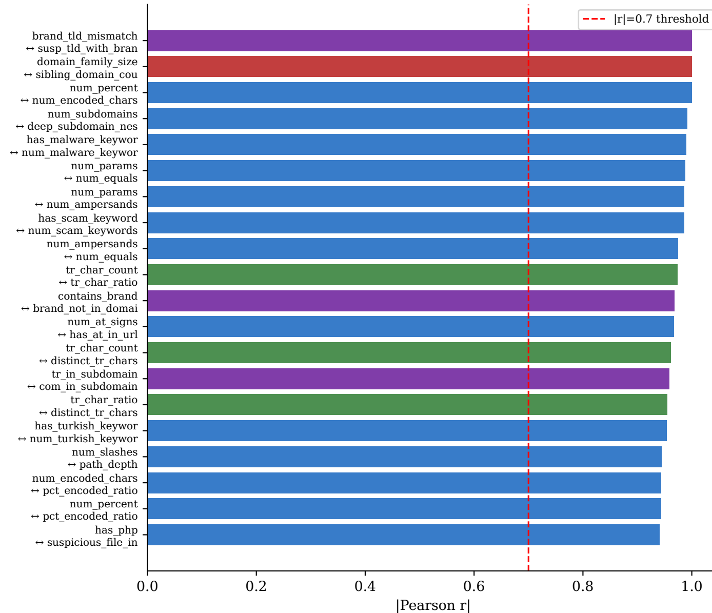
Top-20 Redundant Feature Pairs ( |r| \geq 0.7 )
