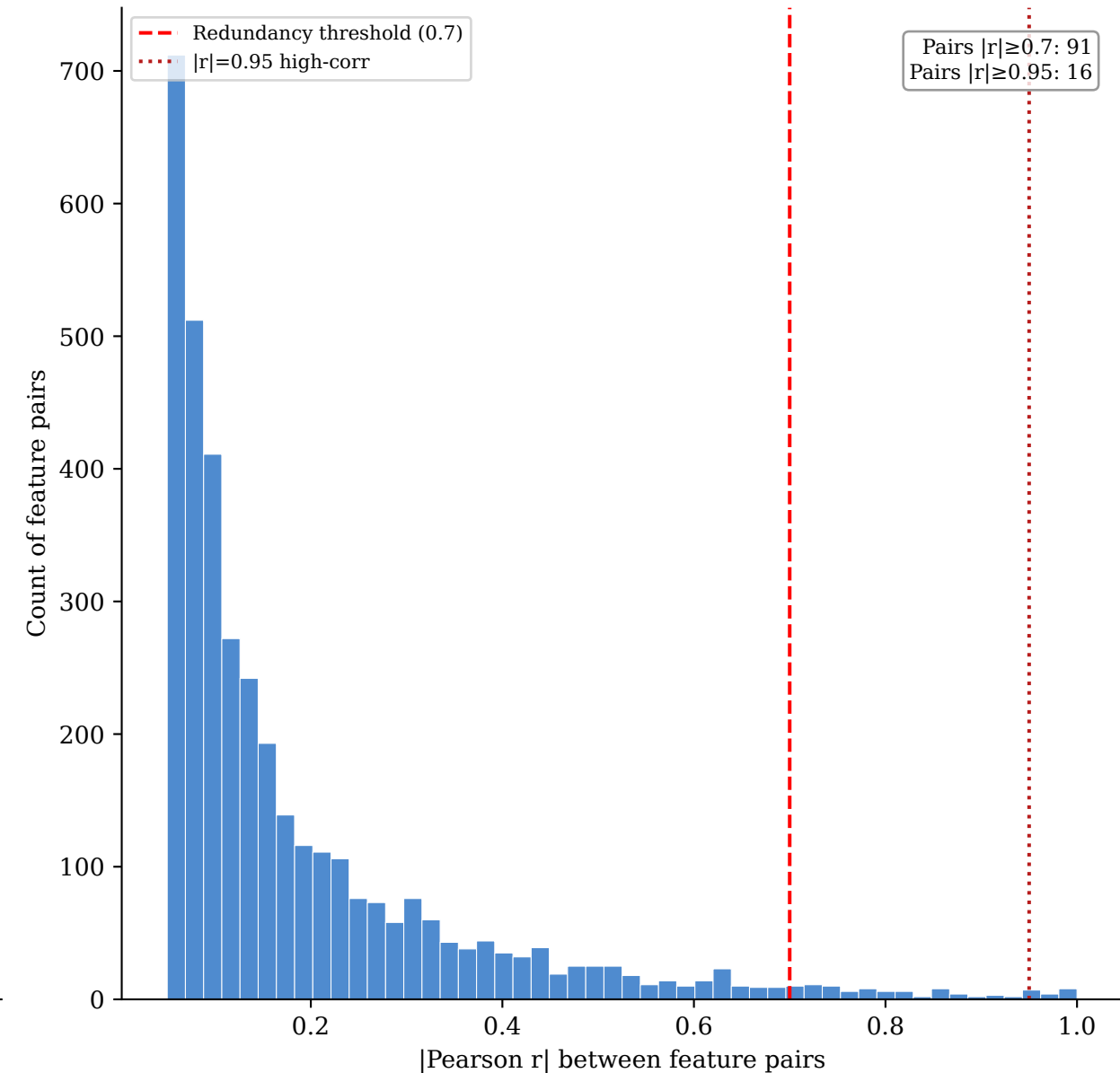
Pairwise |r| Distribution (n=9,045 pairs)
