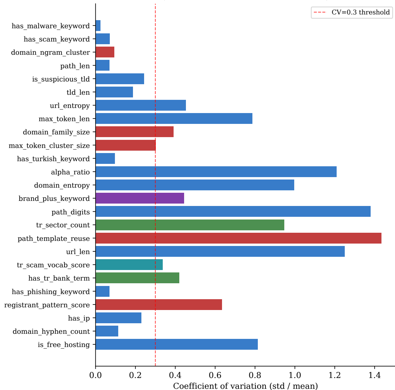
Importance Stability: Coefficient of Variation (lower = more stable across folds)
