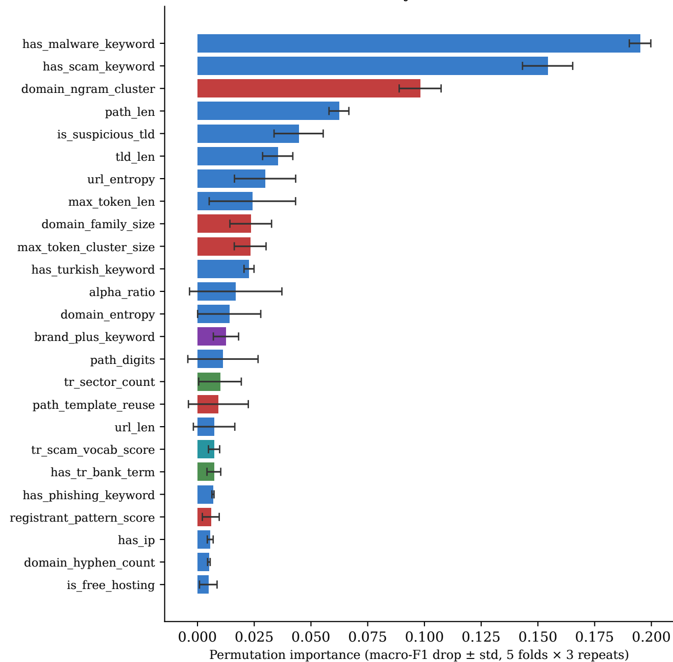
Feature Stability Across 5 CV Folds
