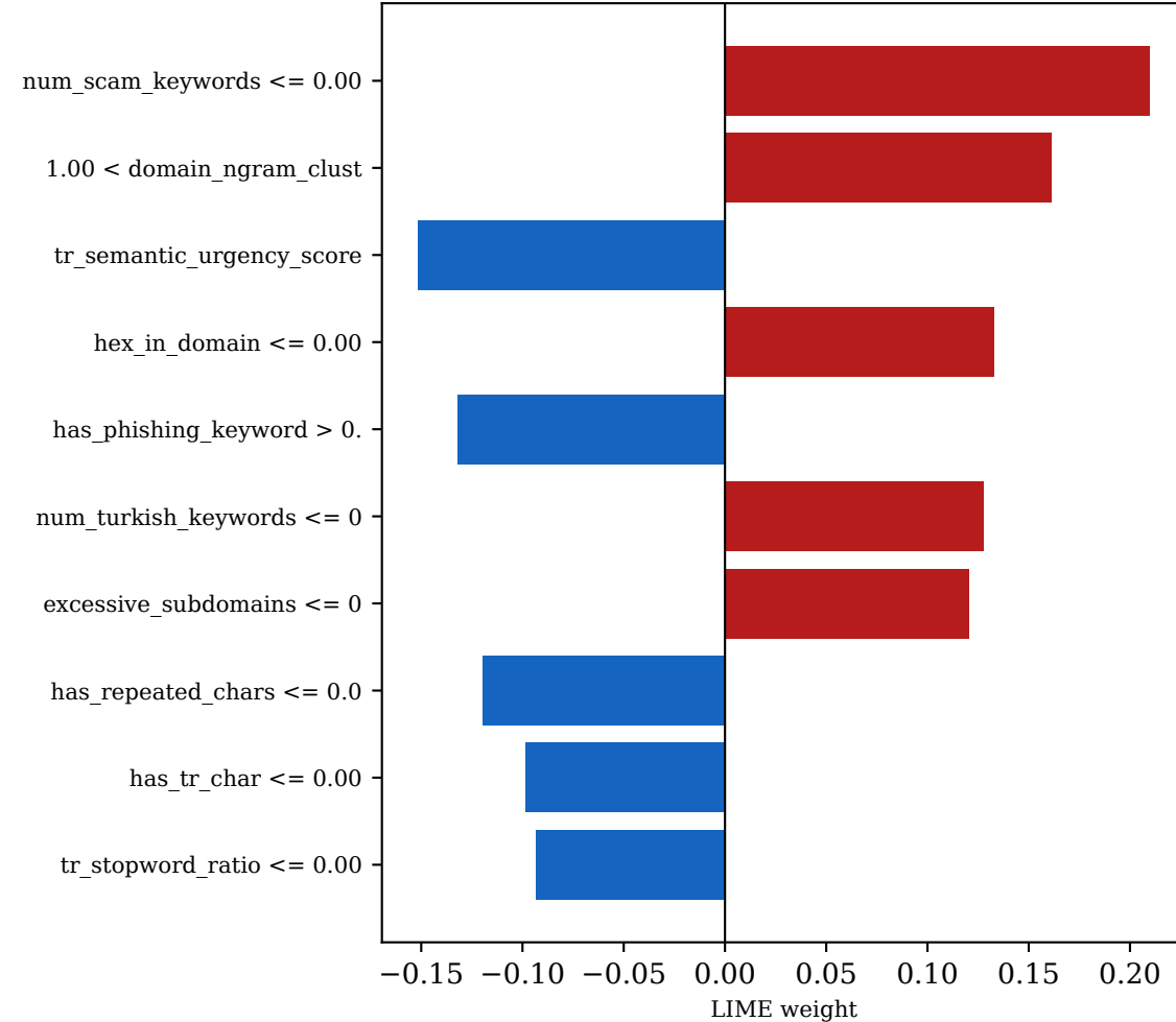
LIME — malicious URL: http://84.203.152.12/recordings/4/www.pa
