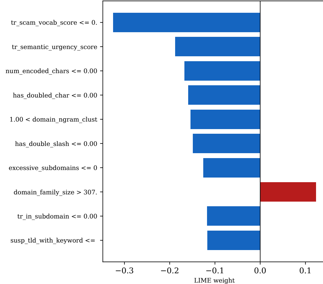
LIME — benign URL: https://akin.av.tr/tag/genel-kurul/
