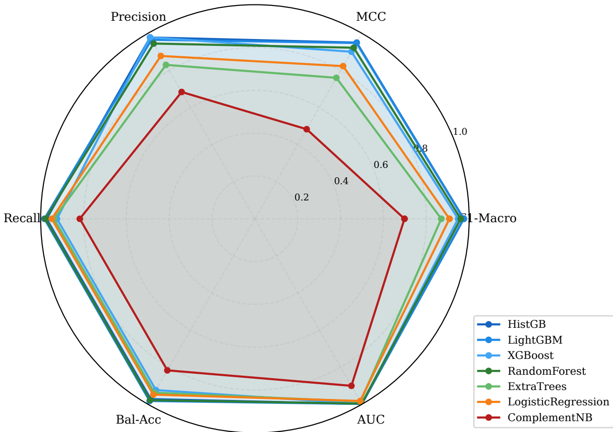
Model Radar Chart — binary (5-fold CV means)
