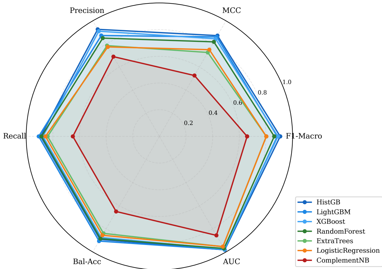
Model Radar Chart — 5class (5-fold CV means)
