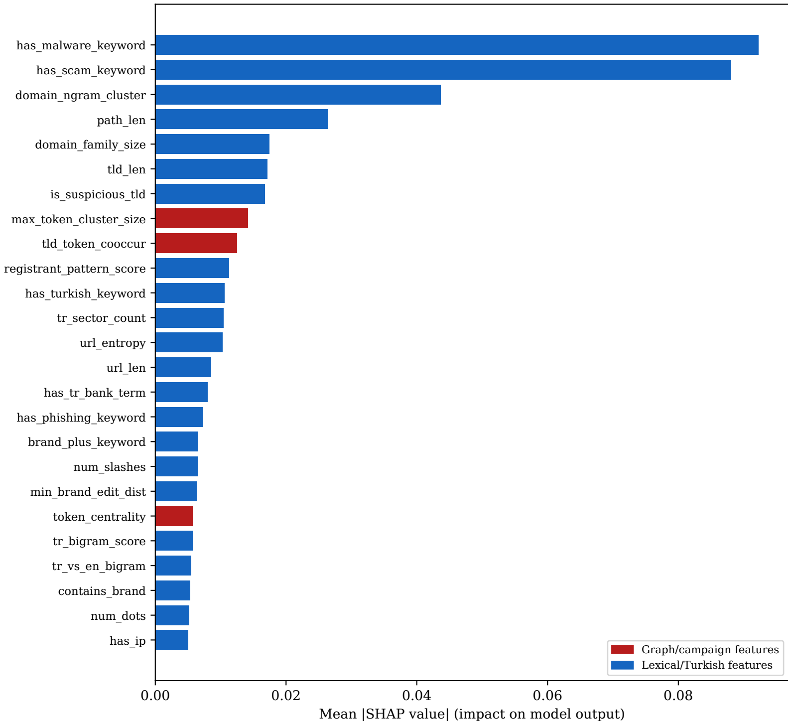
Global Feature Importance — SHAP (5class)
