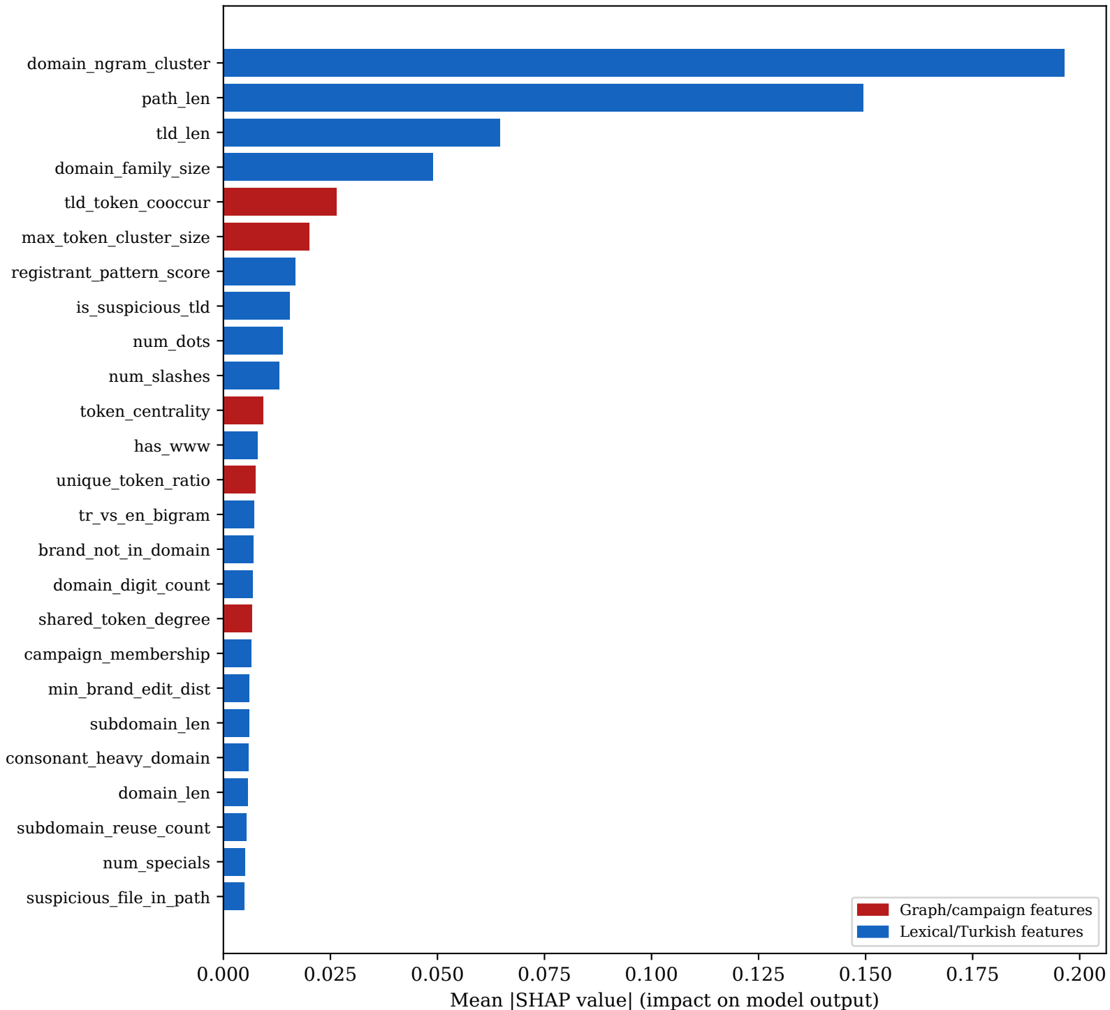
Global Feature Importance — SHAP (binary)
