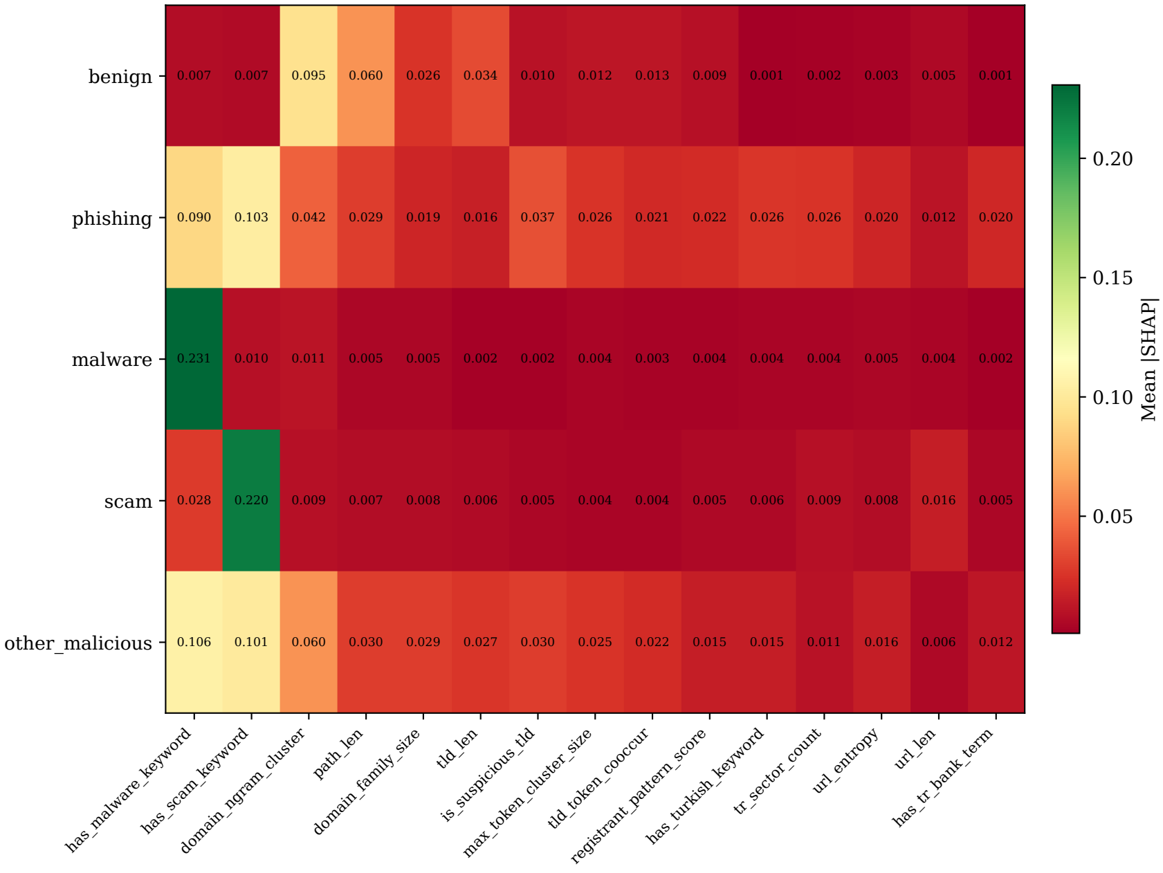
Per-Class SHAP Contribution Heatmap
