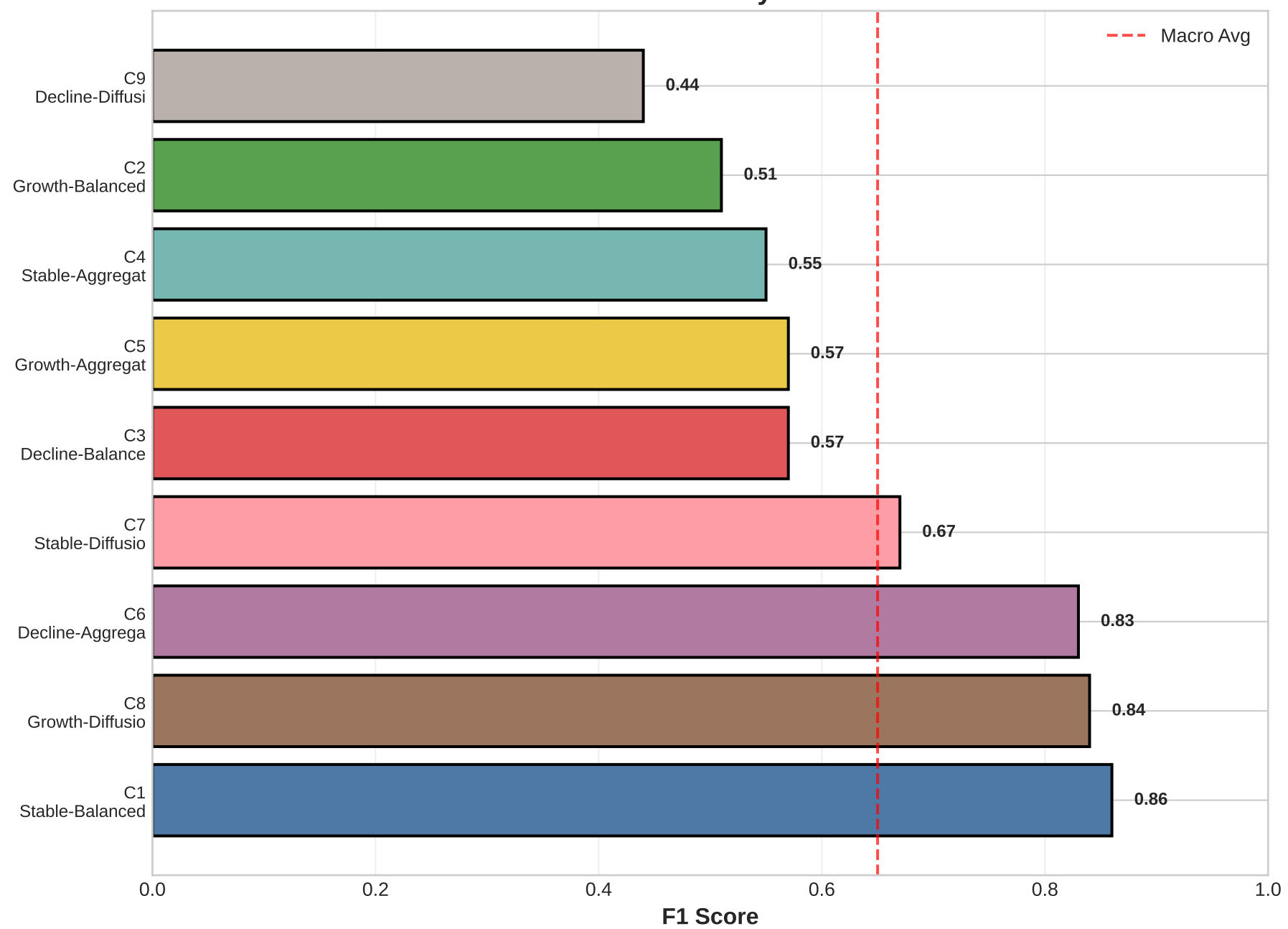
Classes Ranked by F1 Score
