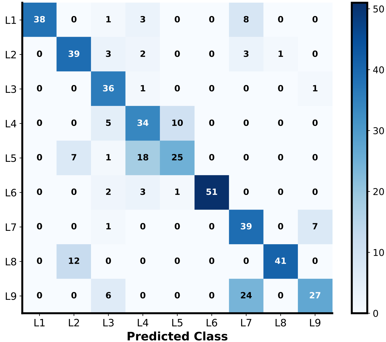
Confusion Matrix (Counts)
