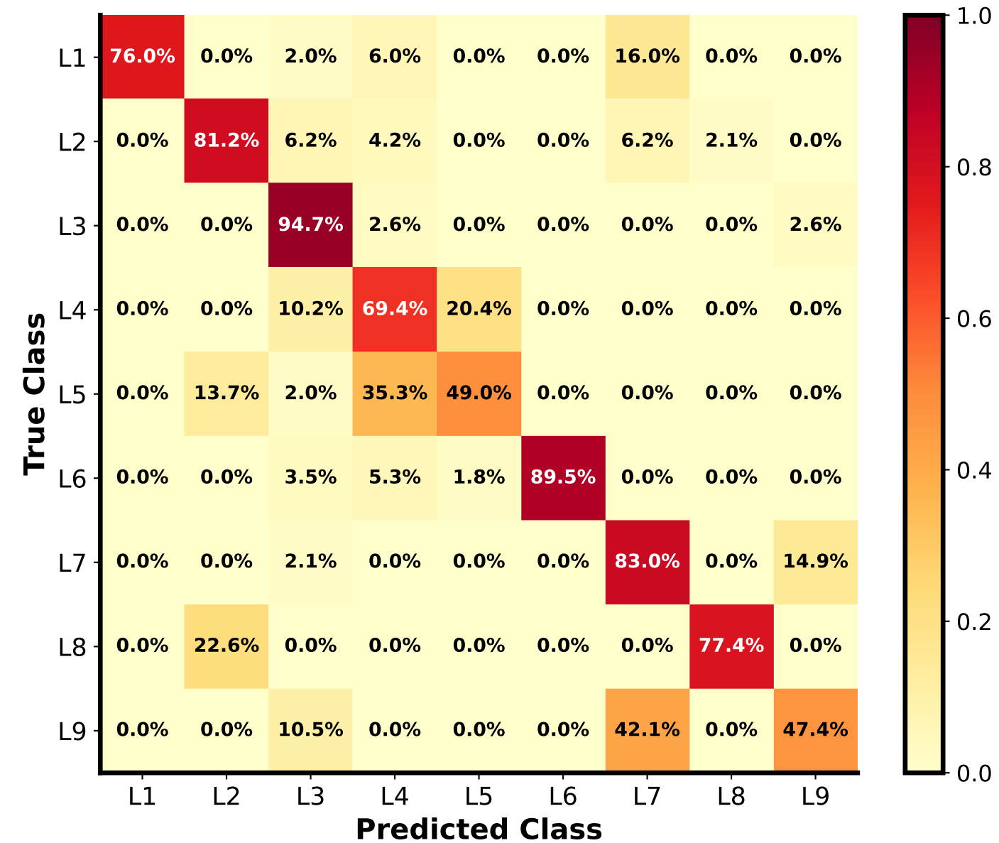
Confusion Matrix (Row-normalised %)
