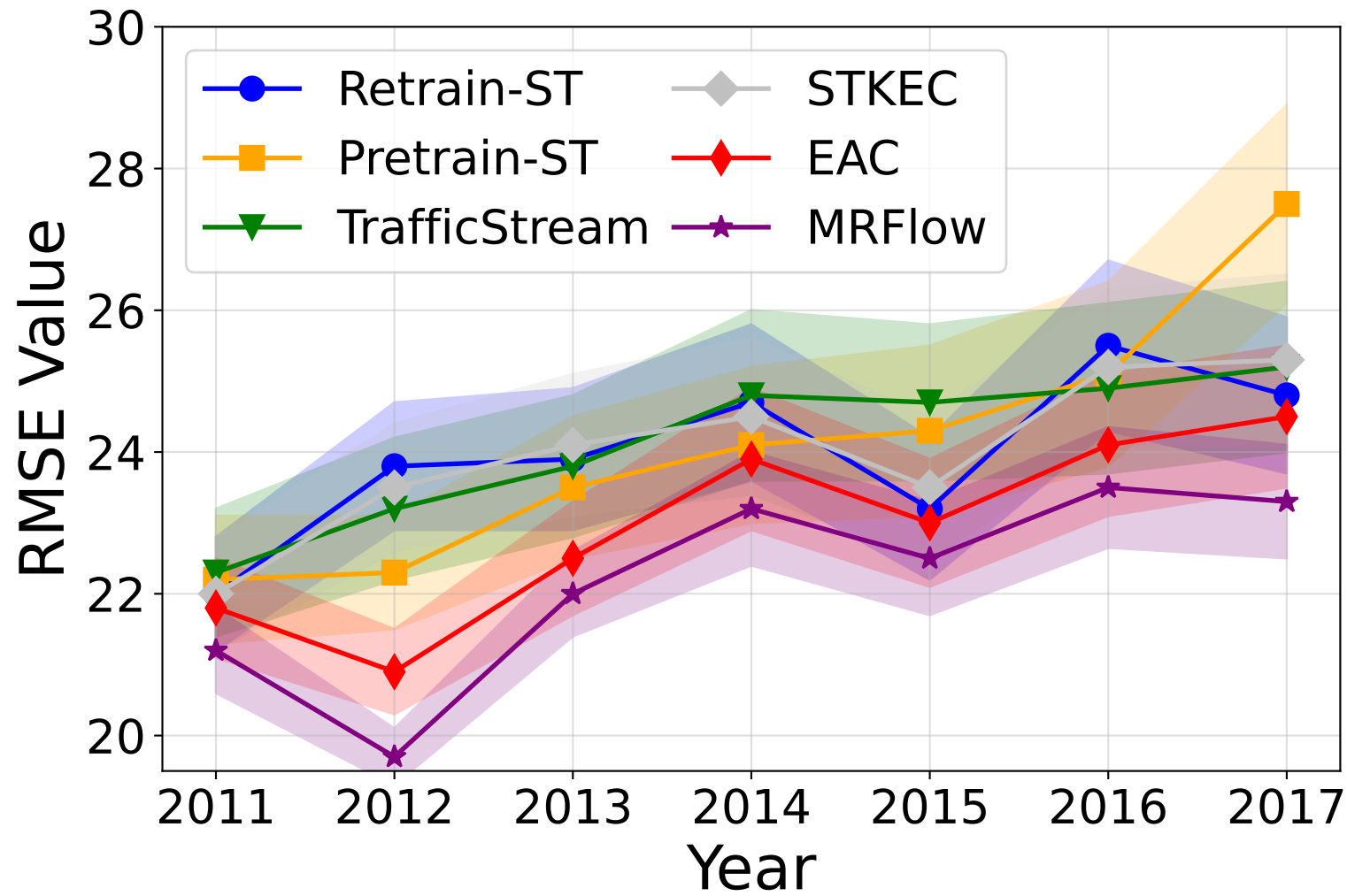
Avg. @ RMSE
