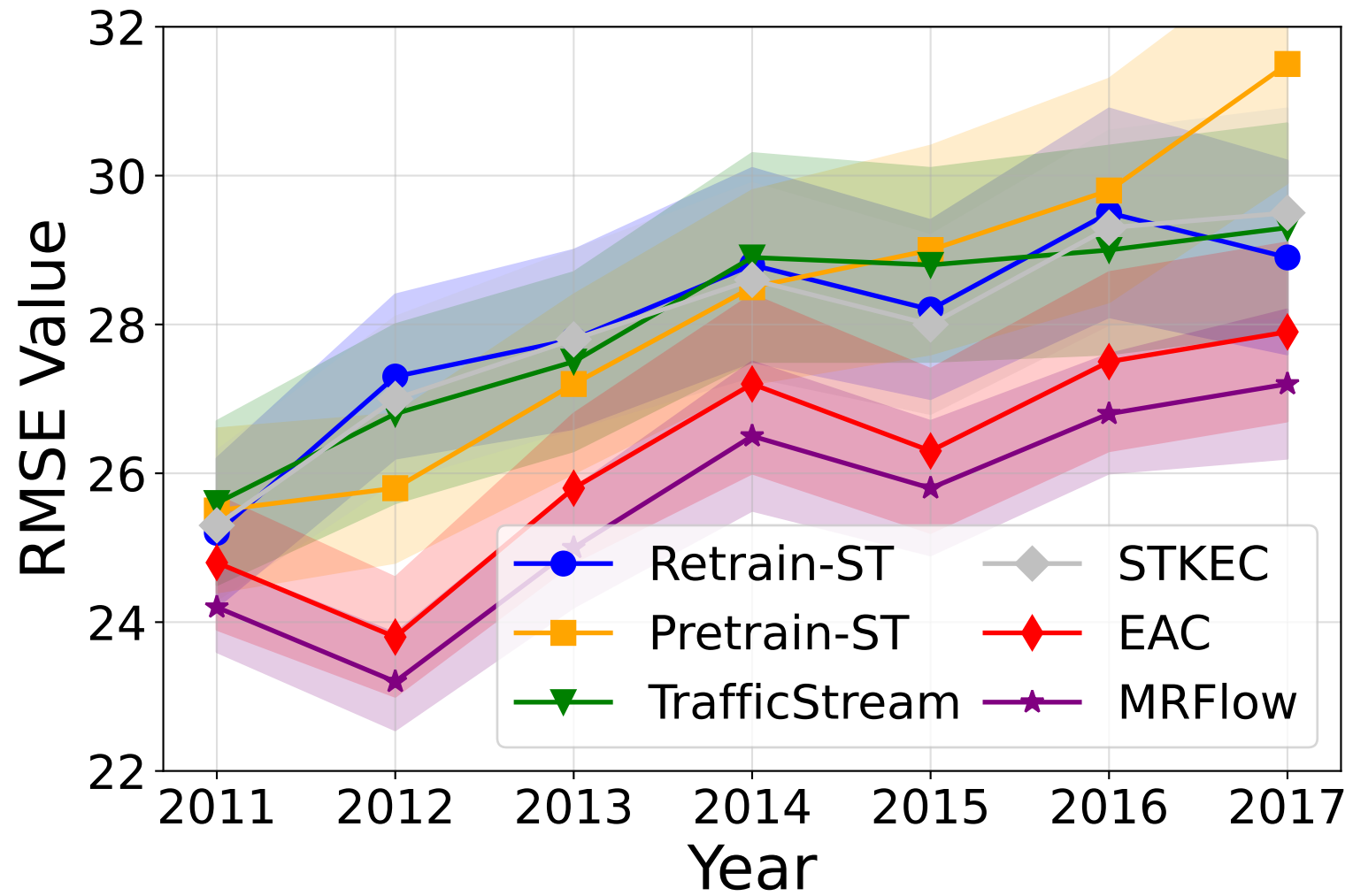
12 @ RMSE
