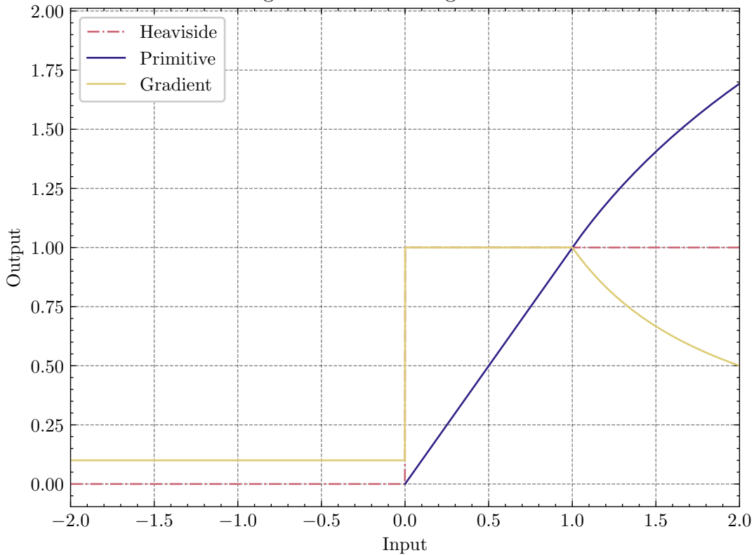
LogTailedReLU surrogate function
