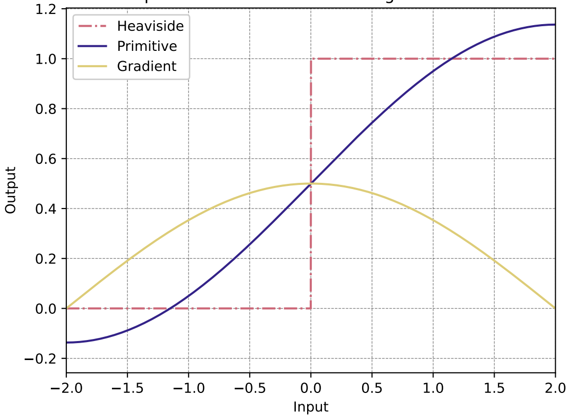
SquarewaveFourierSeries surrogate function
