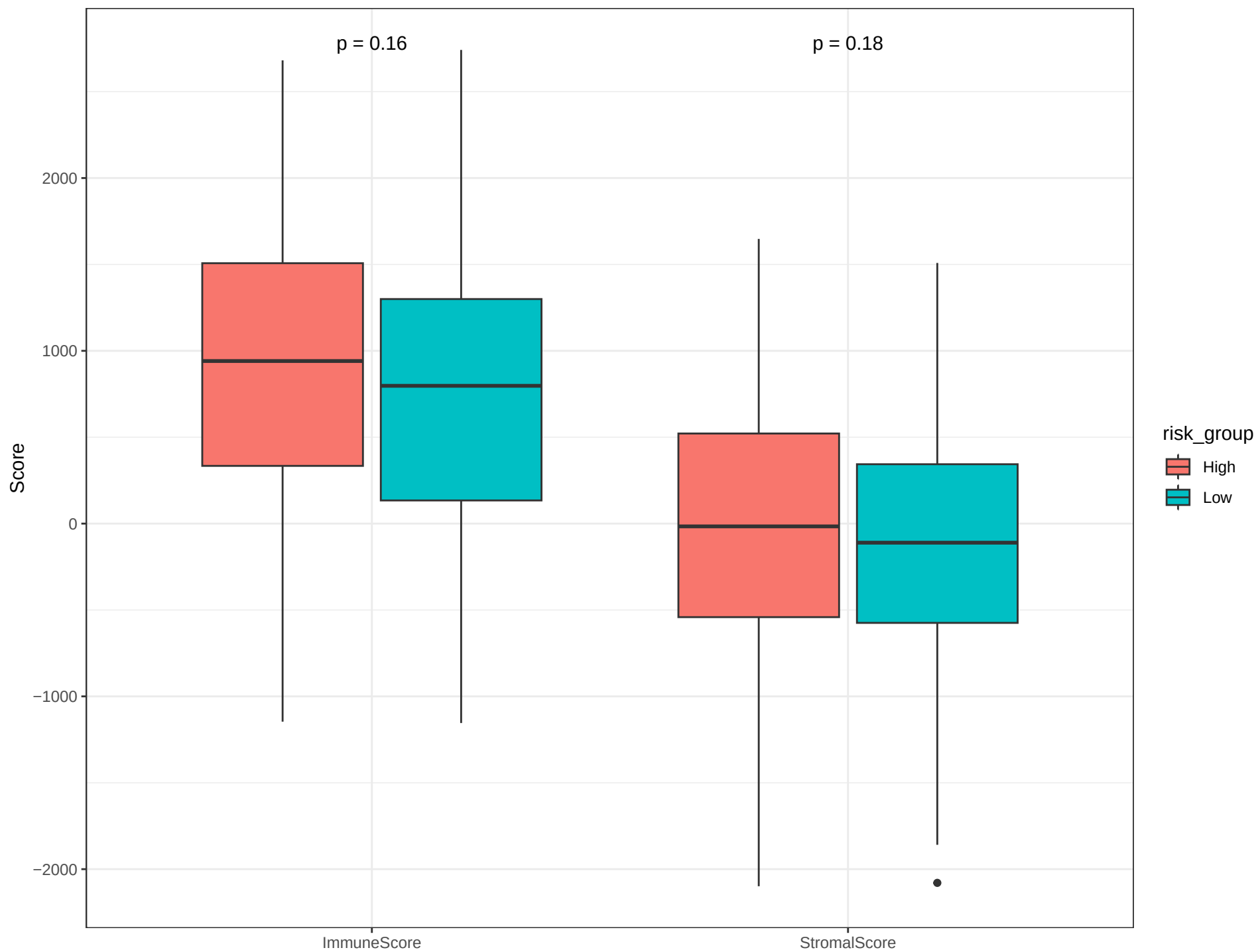
ESTIMATE Immune Score & Stromal Score
