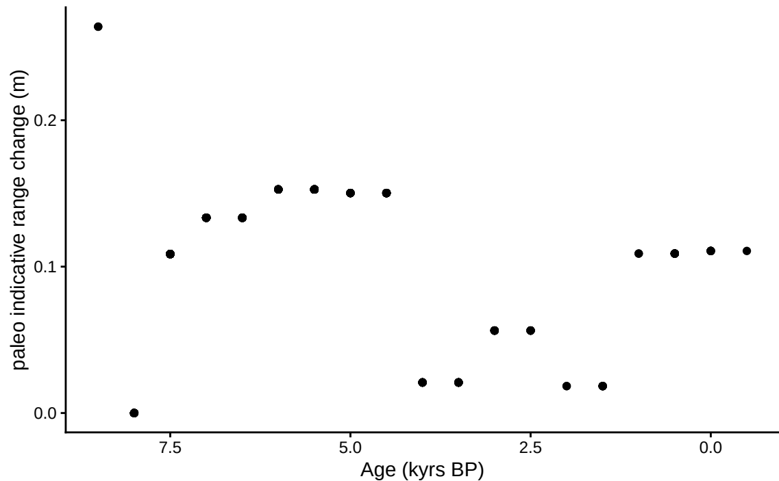
Paleoindicative range change for GR/19/C1 core
