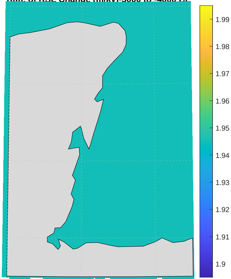
Rate of RSL Change (m/kv)-5000 to -4000 CF
