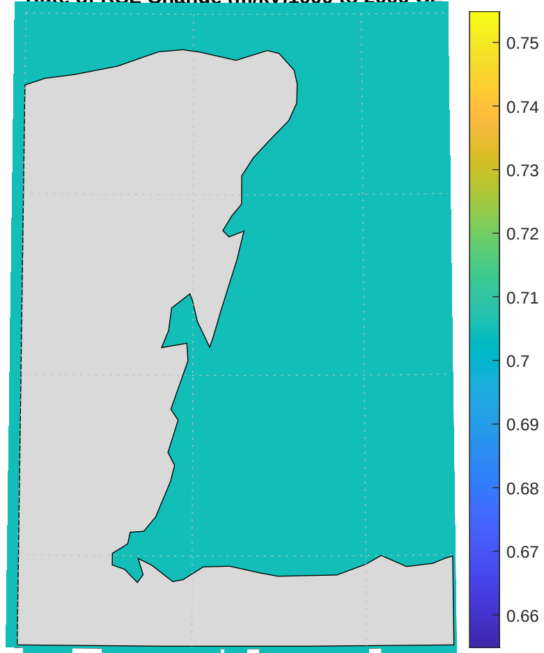
Rate of RSL Change (m/ky)1000 to 2000 CE
