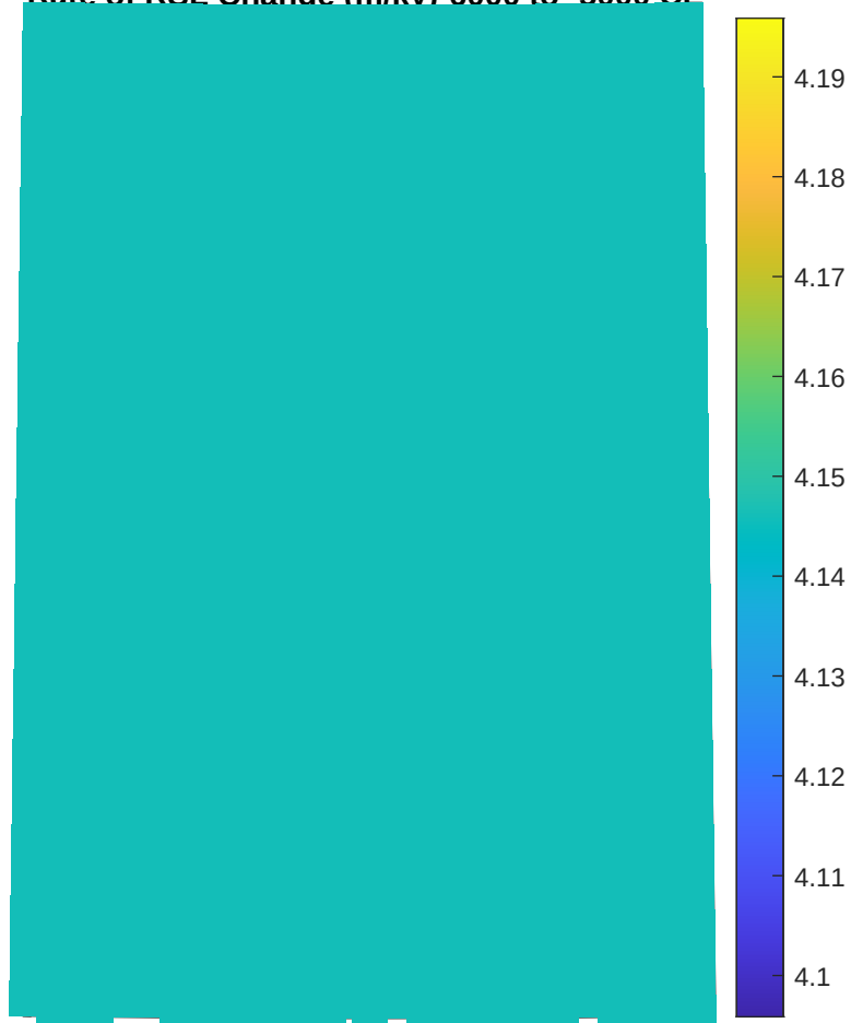
Rate of RSL Change (m/kv)-6000 to -5000 CF
