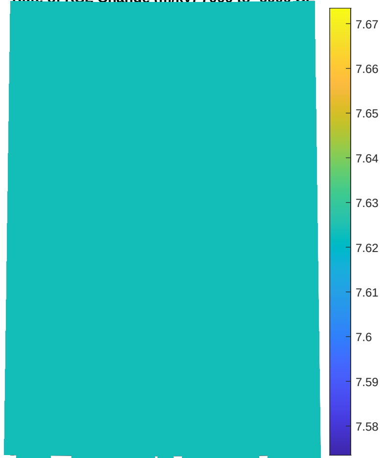
Rate of RSL Change (m/kv)-7000 to -6000 CF
