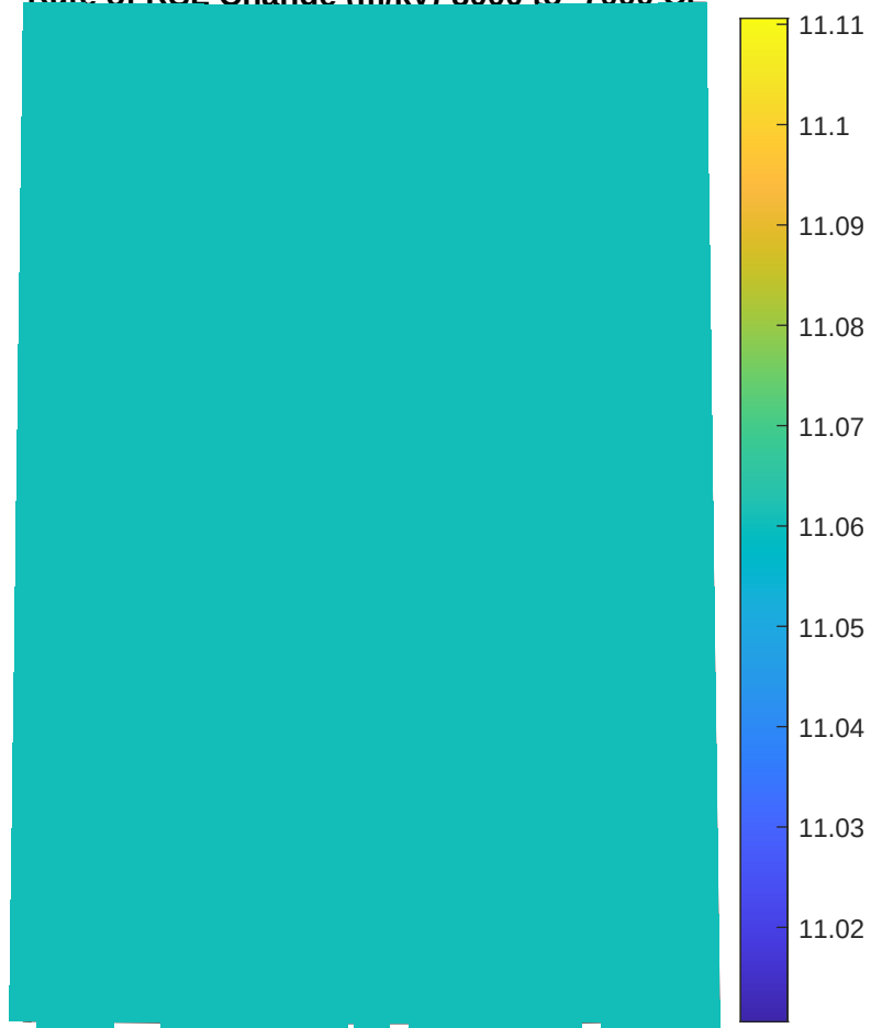
Rate of RSL Change (m/kv)-8000 to -7000 CF
