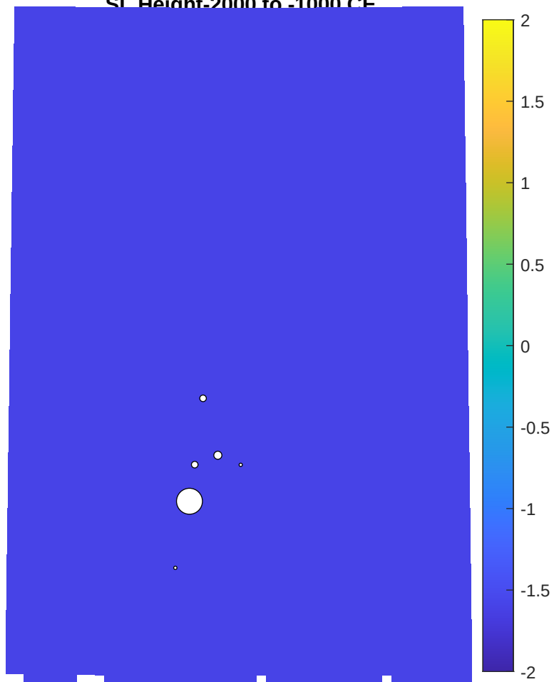
SL Height-2000 to -1000 CE
