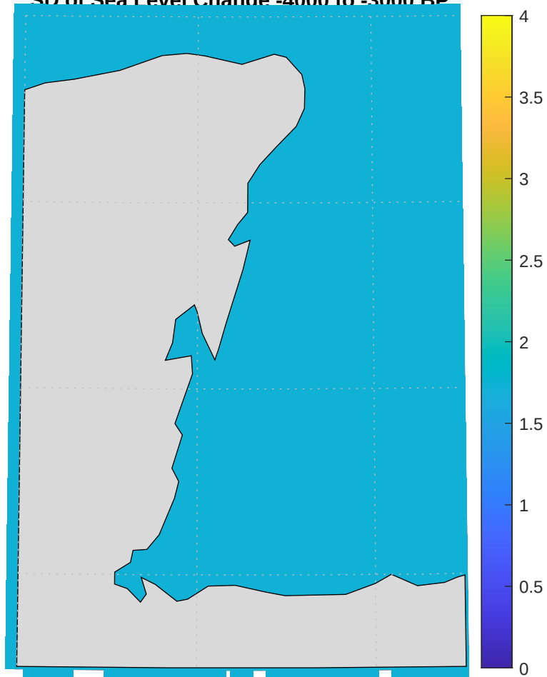
SD of Sea Level Change -4000 to -3000 BP
