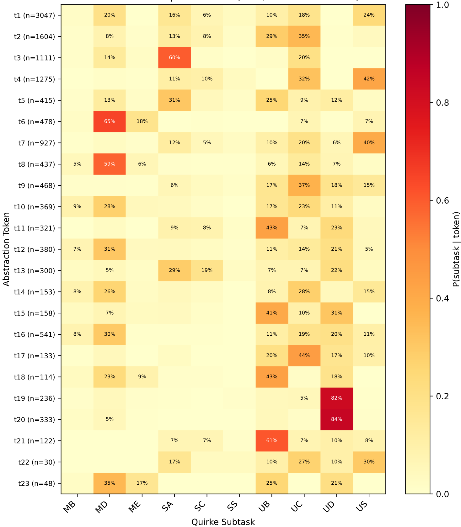
Token--subtask specialization (K=1, codebook size 30)
