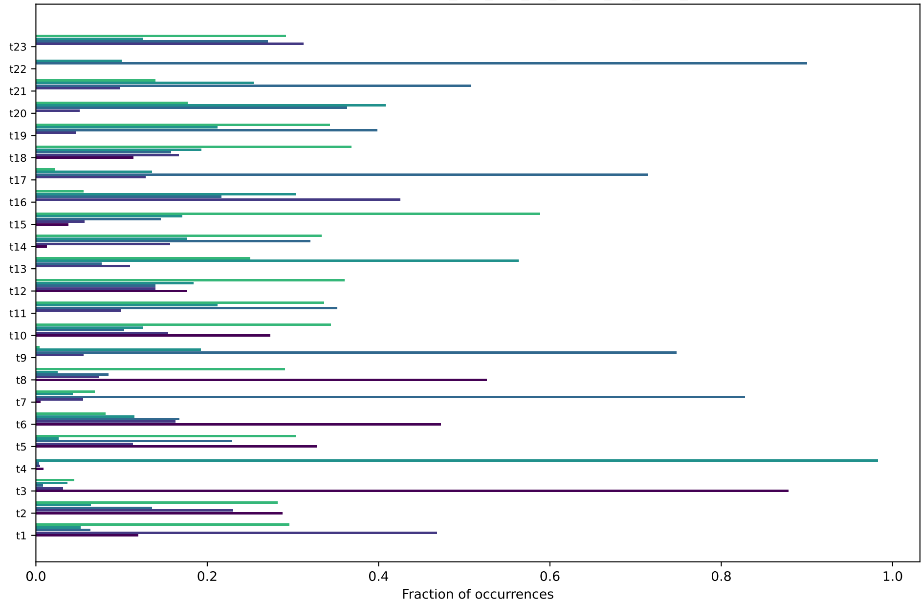
Token Position Distribution — add_sub_sorl_v1_abs30_K1_100K_2L1H128d
