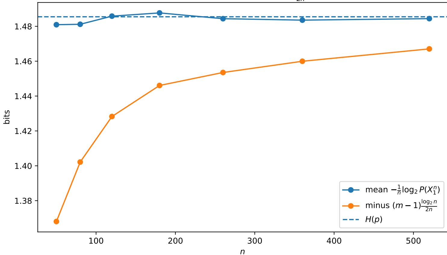
Finite-population: universal (m-1)\frac{\log n}{2n} correction
