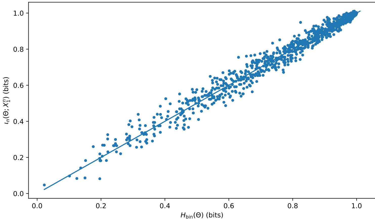
Beta--Bernoulli conditional AEP (n=400, trials=900)
