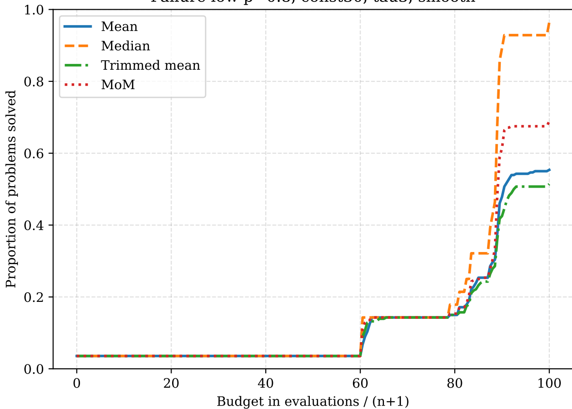
Failure low p=0.8 , const30, tau3, smooth
