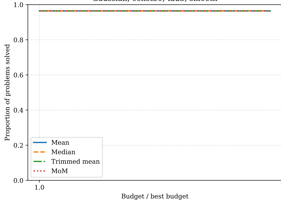
Gaussian, const30, tau3, smooth
