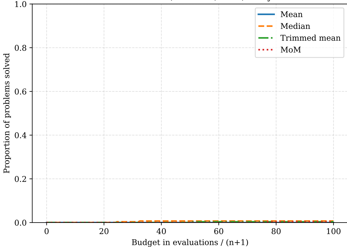
Student-t df1, const30, tau1, noisy
