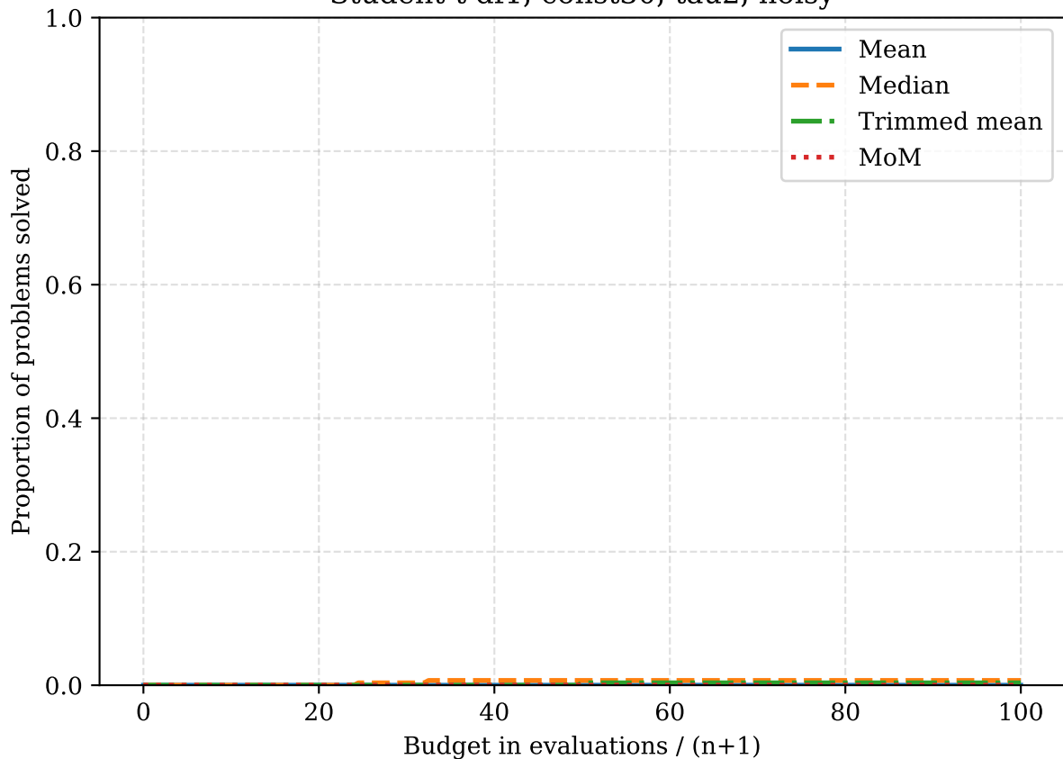
Student-t df1, const30, tau2, noisy
