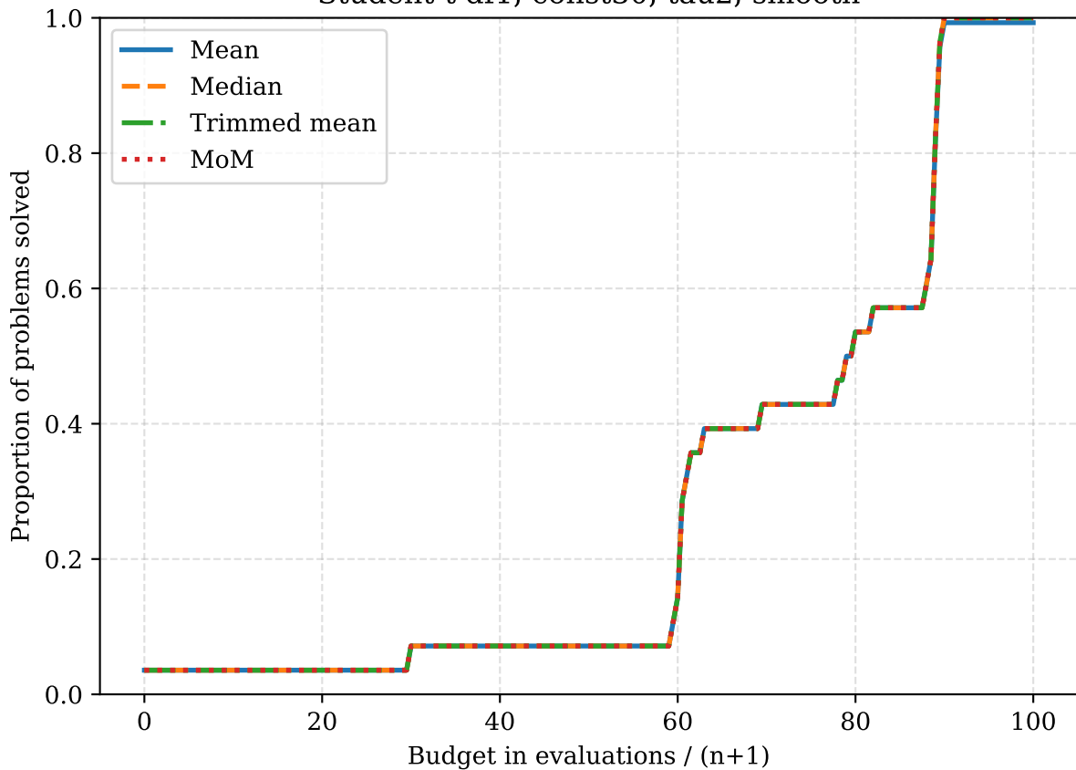
Student-t df1, const30, tau2, smooth
