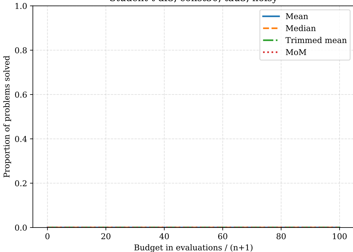
Student-t df3, const30, tau3, noisy
