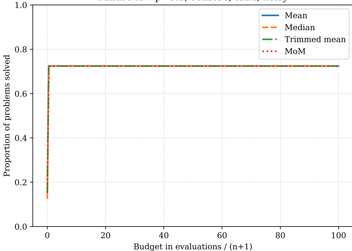
Failure low p=0.8 , const30, tau4, noisy
