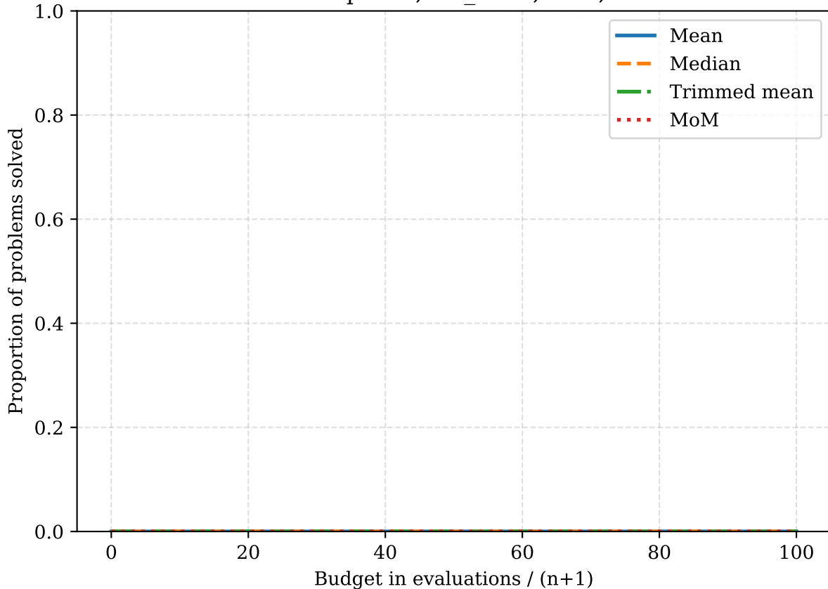
Failure low p=0.8 , inv_delta, tau4, smooth
