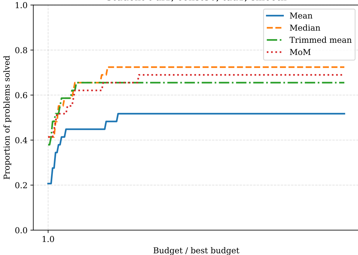
Student-t df1, const30, tau1, smooth
