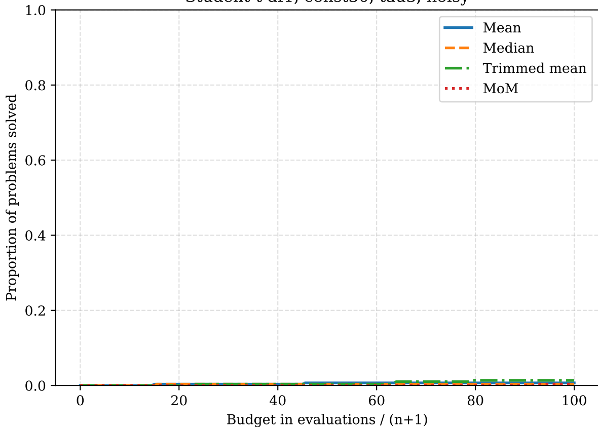
Student-t df1, const30, tau3, noisy
